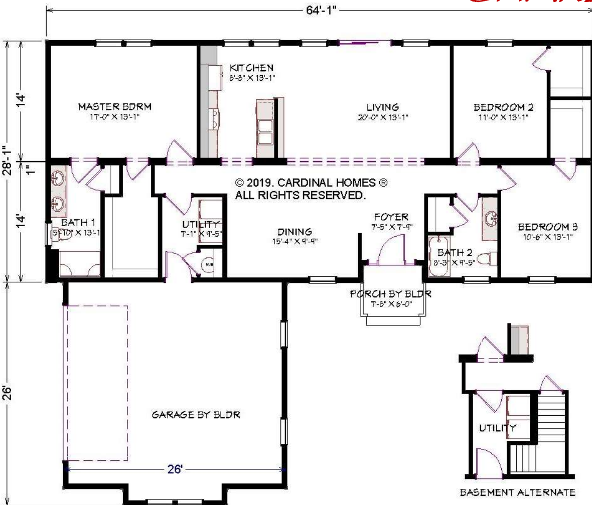
FLOOR PLAN Matches Elevation A rendering
