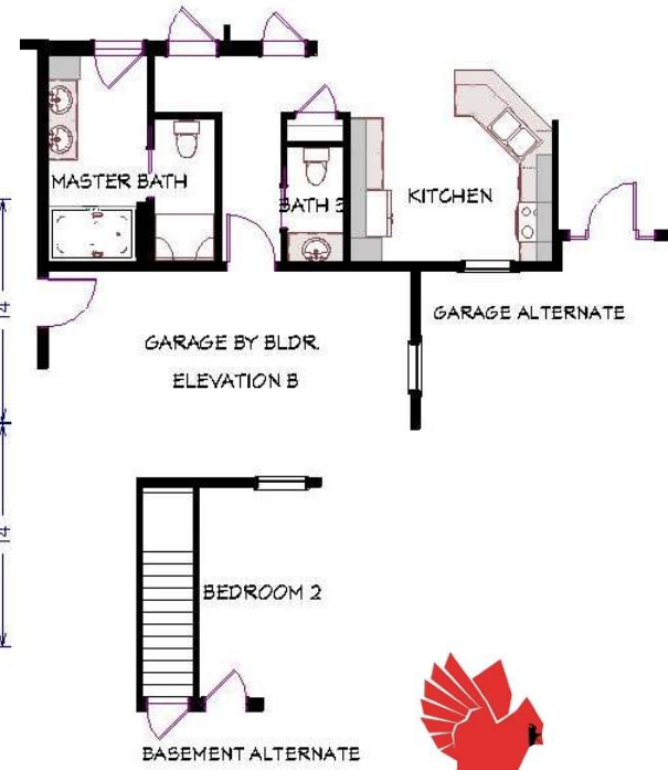
FLOOR PLAN Matches Elevation A rendering
