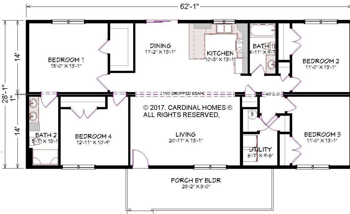
FLOOR PLAN Matches Elevation B rendering
