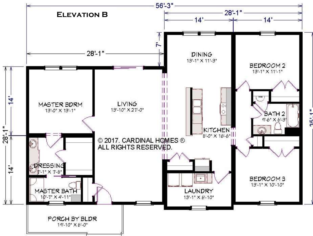
FLOOR PLAN Matches Elevation B rendering
