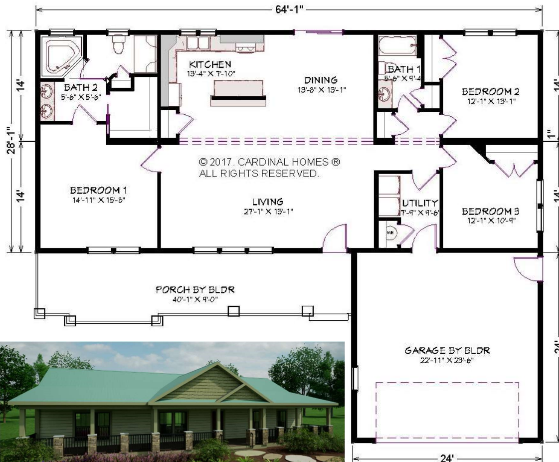
FLOOR PLAN Matches Elevation A rendering
